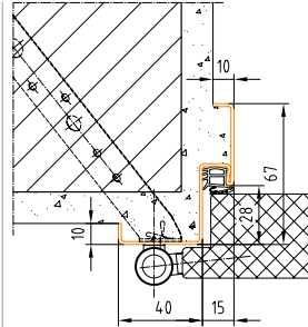
Profil 22_M - str. 9, 15, 21 BRMB = DLB + 50 mm BRMH = DLH + 25 mm
